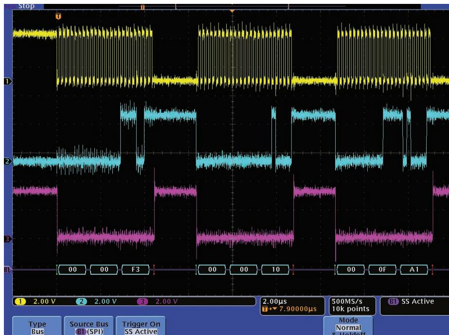
Figure 13. Correct synthesizer configuration messages.
