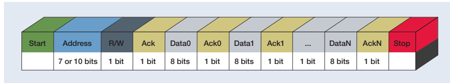
Figure 4. I 2 C message structure.
