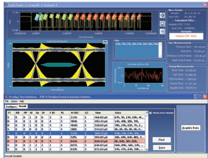
Figure 36. Eye Diagram analysis of a FlexRay signal.
