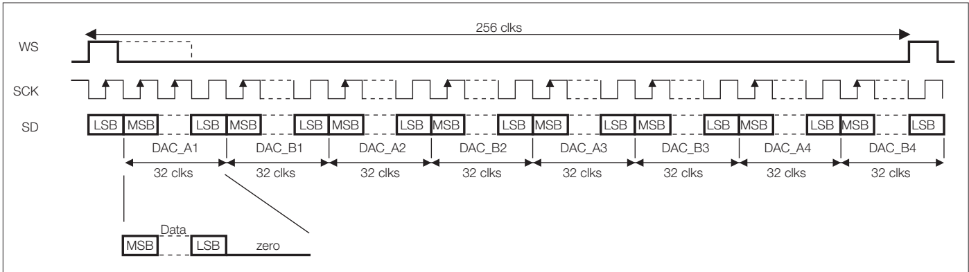
Figure 40. TDM Format.
