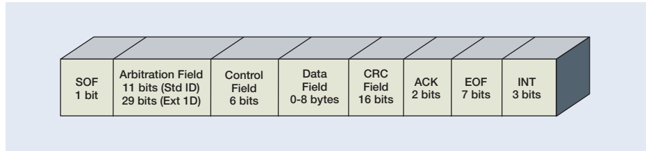
Figure 26. CAN Data/Remote Frame.
