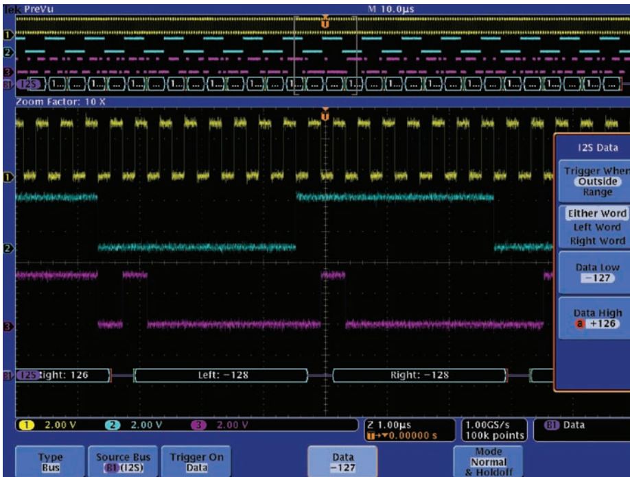
Figure 41. Triggering outside a range of values on an I 2 S bus.
