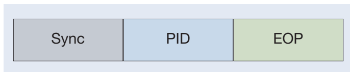
Figure 18. Handshake packet organization.
