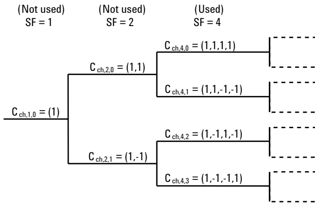
Figure 22. Code tree generation of OVFSF codes
