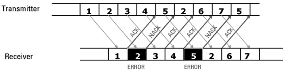
Figure 34a. HARQ uses link-layer acknowledgments to make re-transmission decisions
