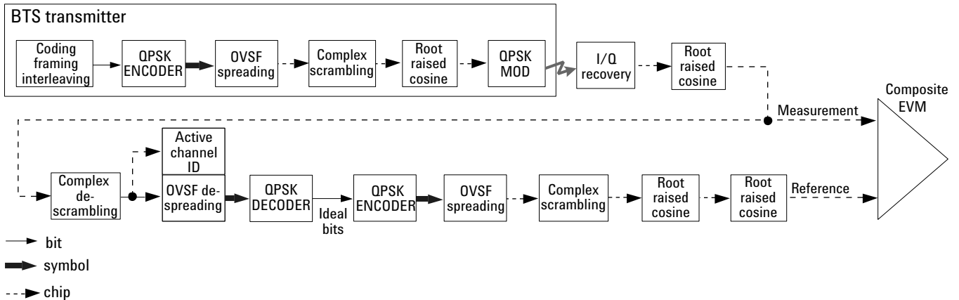
Figure 20. Process to calculate composite EVM for a W-CDMA DL signal
