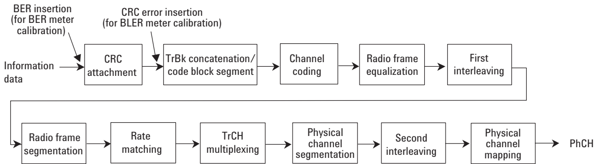
Figure 36. BER and BLER meter calibration
