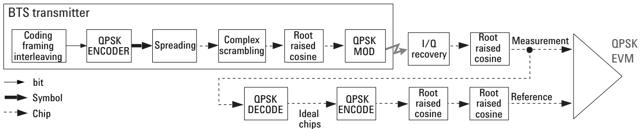
Figure 18. Process to calculate QPSK EVM for a W-CDMA DL signal
