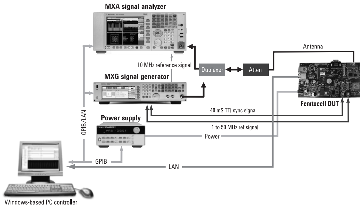
Figure 42. Typical femtocell production test station
