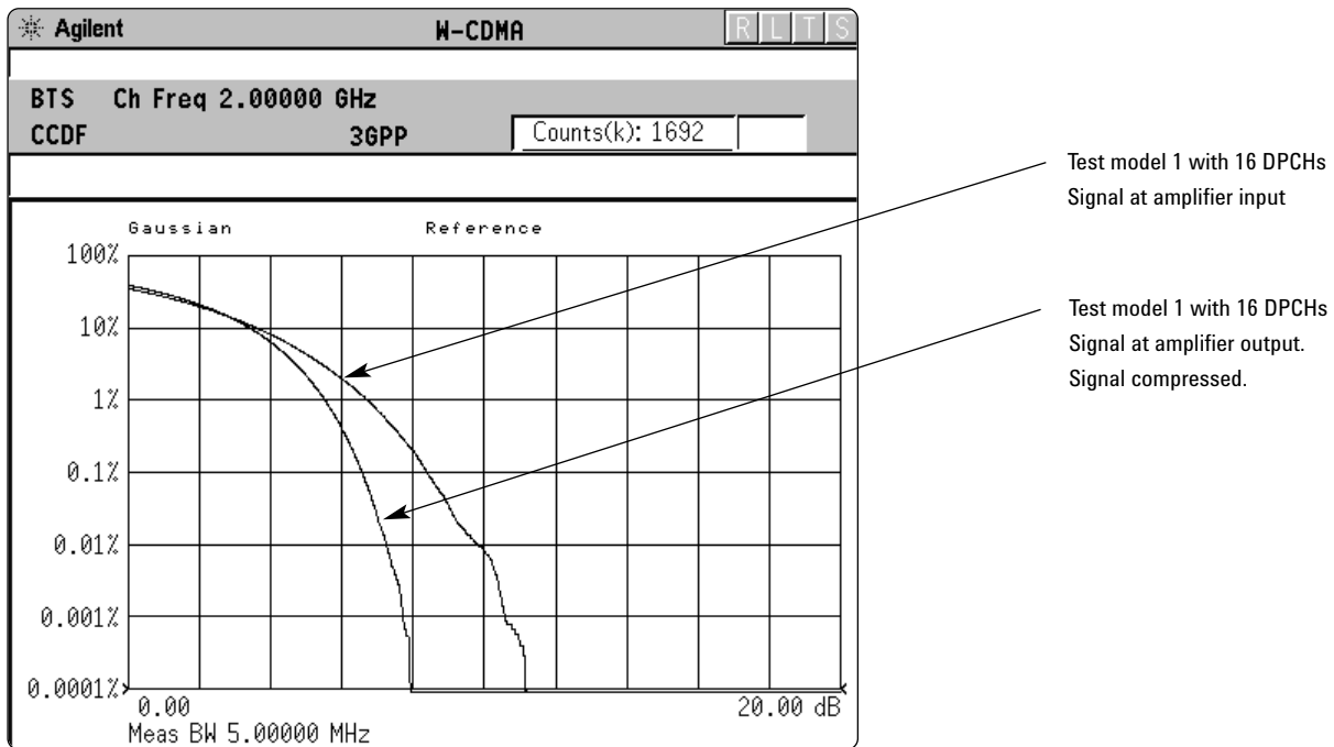
Figure 15. CCDFs for test model 1 with 16 code channels with and without compression
