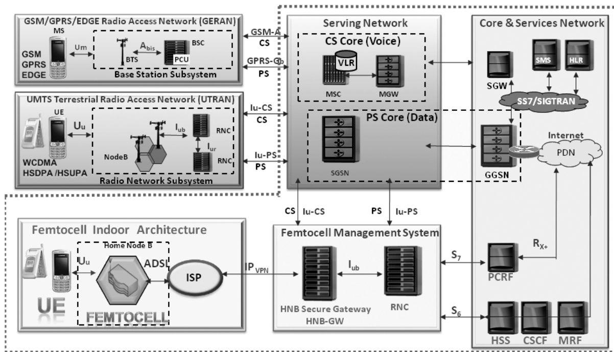
Figure 39. Typical network implementation with femtocell management
