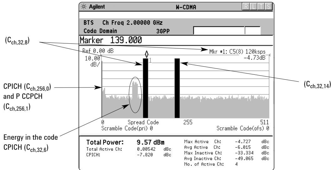
Figure 25. Code domain power display for a signal with the P CCPCH/SCH, CPICH, and two DPCHs ( C_{ch,32,8} and C_{ch,32,14} ).
