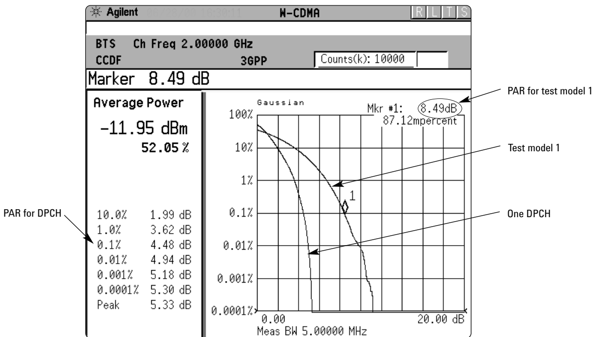
Figure 14. CCDF of a W-CDMA signal with one DPCH and a signal configured as test model one with 16 DPCHs
