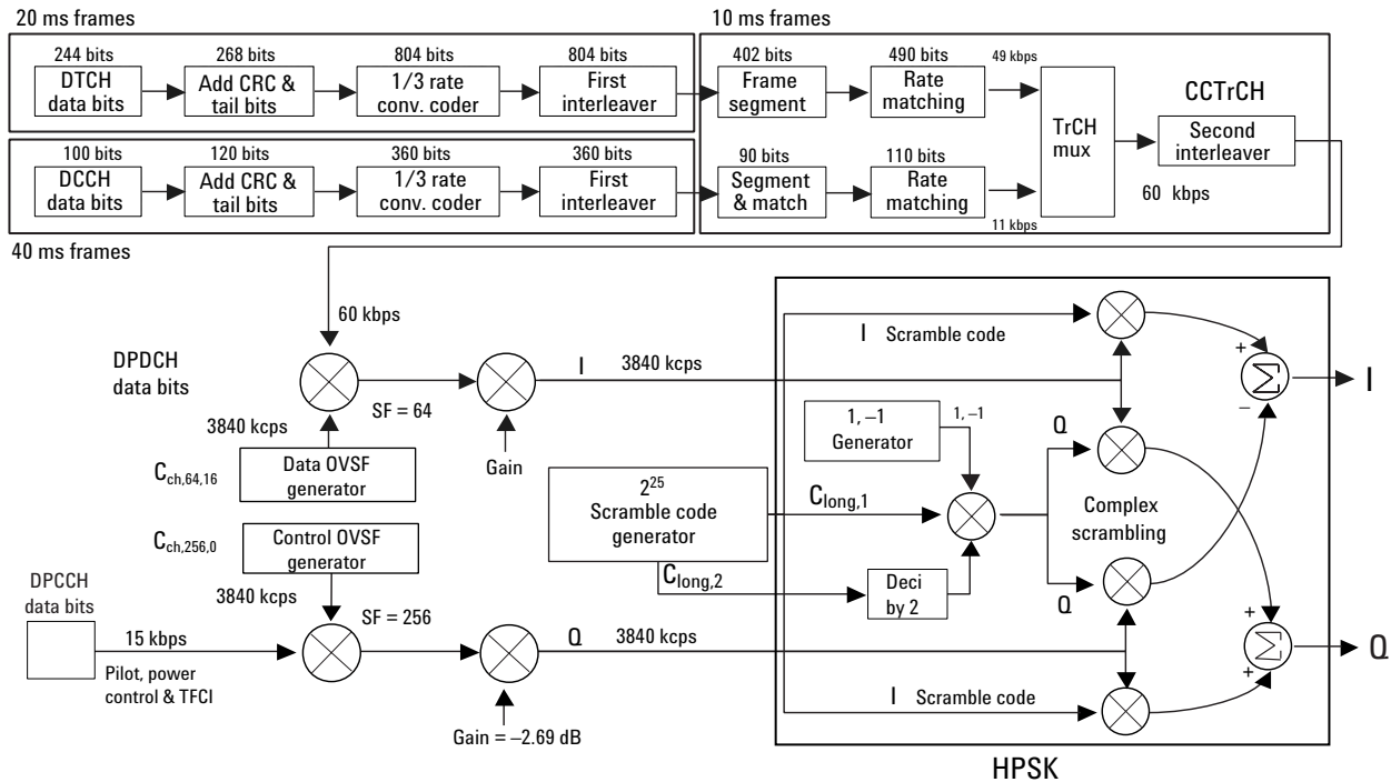
Figure 11. Uplink DPCH/DPCCH coding, spreading, and scrambling.
