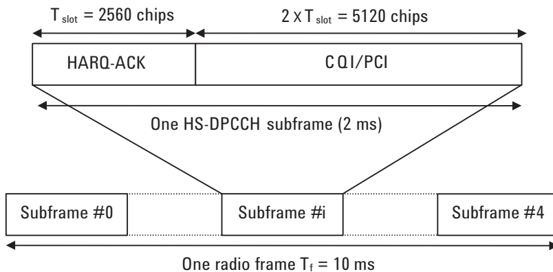
Figure 9a. Frame structure for uplink HS-DPCCH
