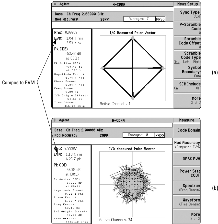
Figure 21. Vector diagram and composite EVM measurement for a W CDMA DL signal with (a) the P CCPCH/SCH, and (b) the P CCPCH/SCH, CPICH, and 32 DPCHs.
