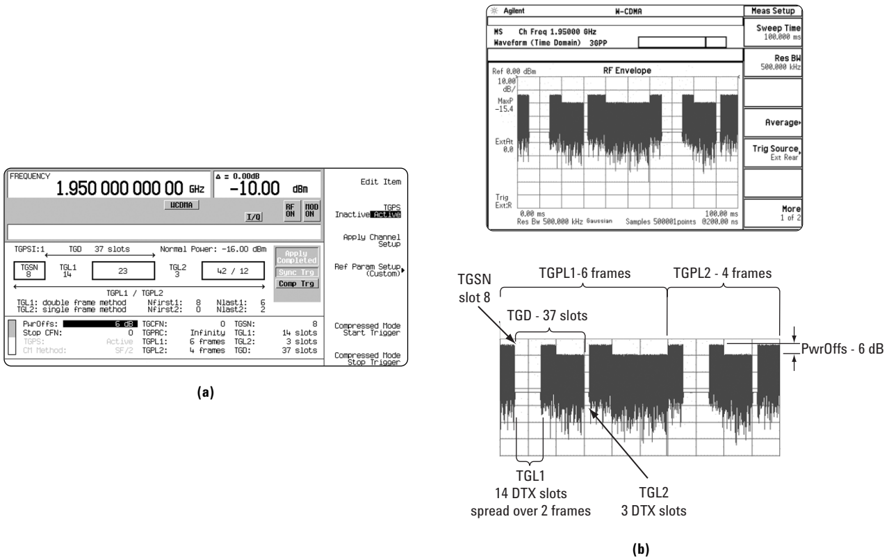
Figure 37. (a) Compressed mode setup and (b) Displayed compressed signal
