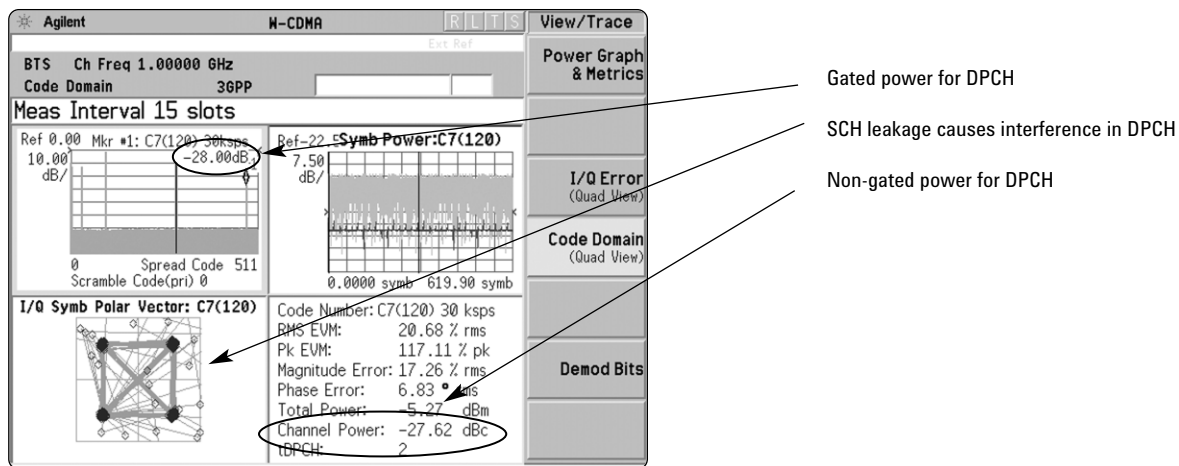
Figure 33. Gated and non-gated power for DPCH for power control dynamic range
