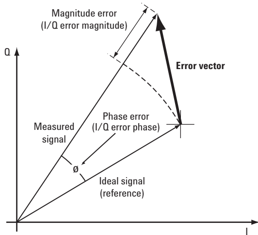
Figure 16. Error vector and related parameters
