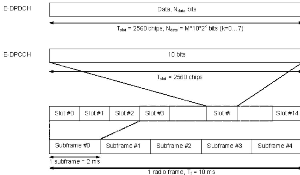
Figure 9b. E-DPDCH frame structure
