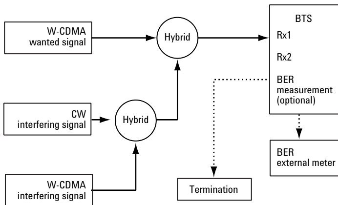
Figure 35. General setup for receiver characteristics tests
