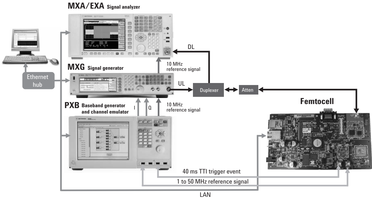
Figure 40. Example of femtocell Tx/Rx RF test setup for R&D
