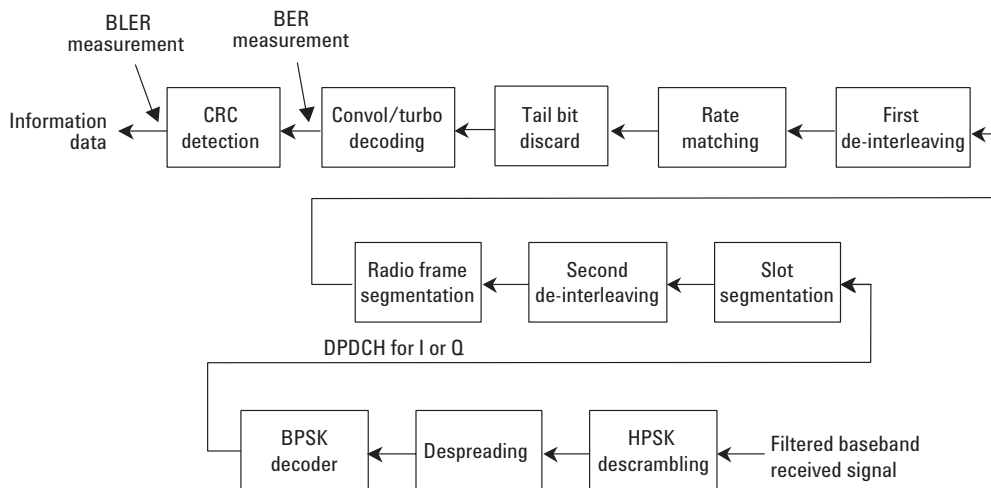
Figure 34. BER and BLER measurements in the W-CDMA BTS receiver chain for a DPDCH.
