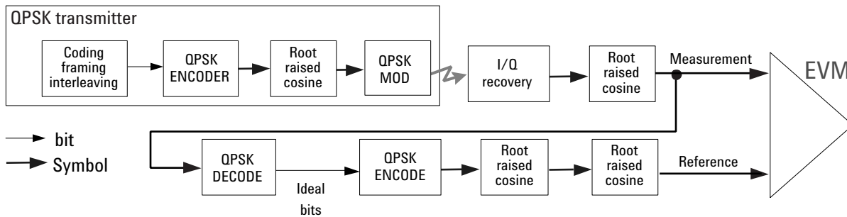
Figure 17. Process to calculate EVM for a generic QPSK signal
