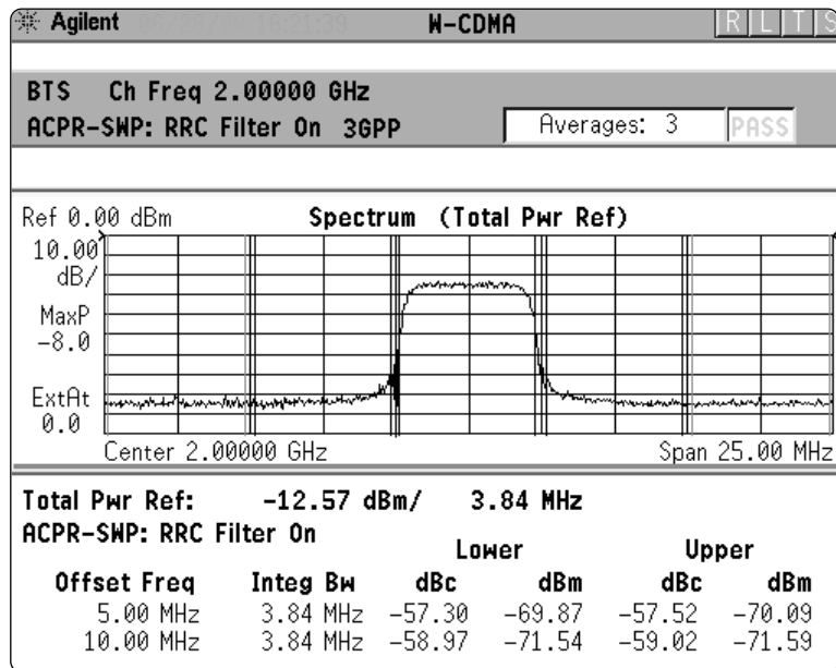
Figure 13. ACLR measurement for test model 1 with 16 DPCHs.
