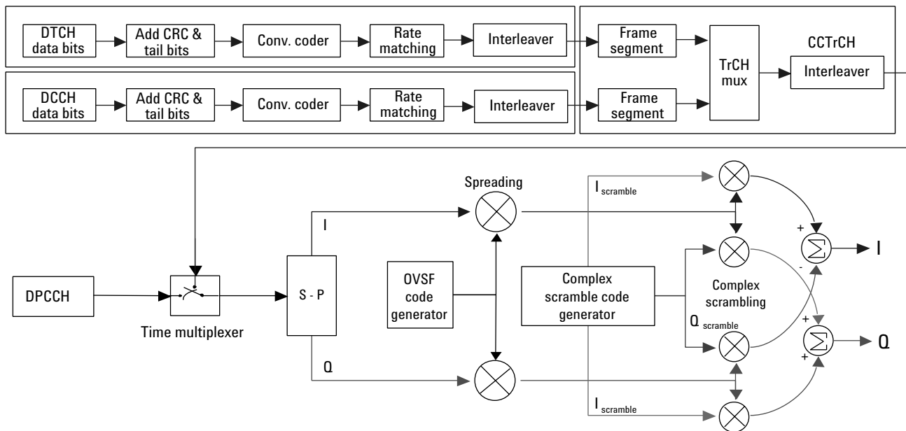
Figure 10. Downlink DPDCH/DPCCH coding, spreading, and scrambling.
