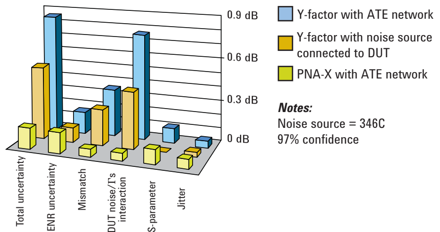
Uncertainty contributors
