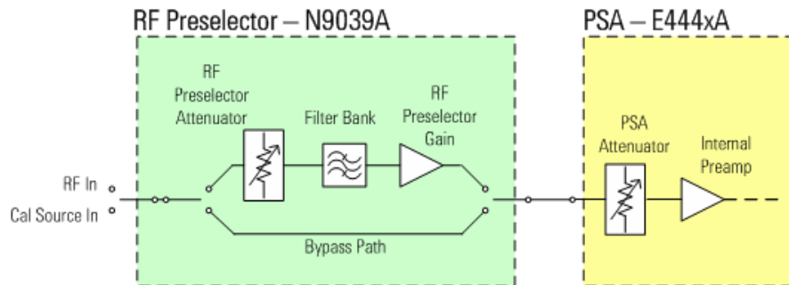
Figure 24-1 EMI Receiver Block Diagram
