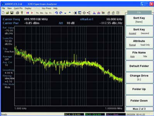
Phase Noise
