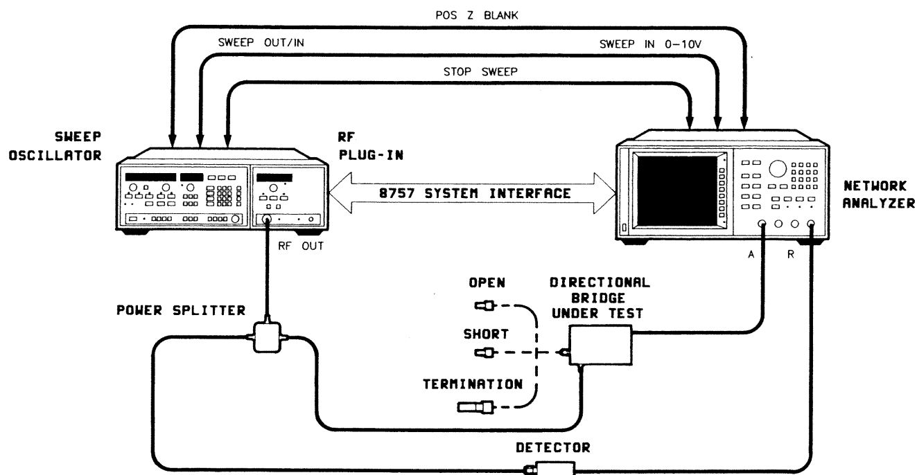
Figure 4-1. Directivity Test Setup 0.01 to 4 GHz
