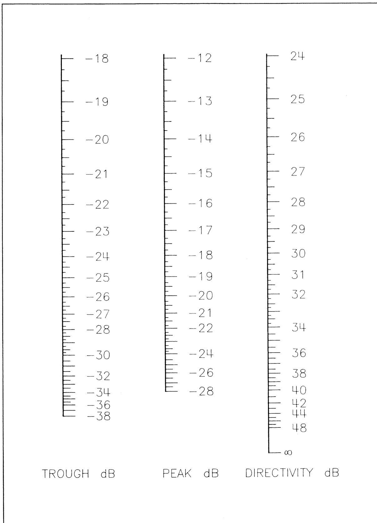
Figure 4-5B. Directivity Nomogram
