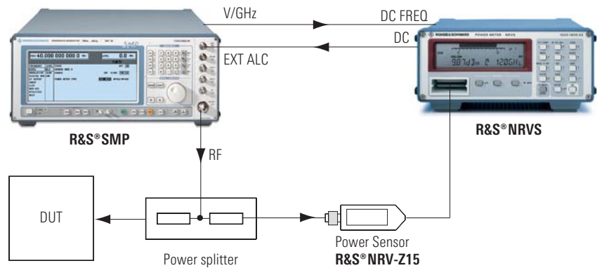
FIG 7: External level control for the Microwave Signal Generator R&S®SMP
