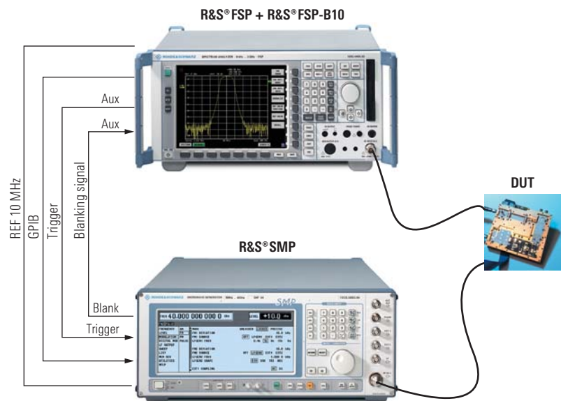
FIG 8: Scalar network analysis with the Microwave Signal Generator R&S®SMP and the Spectrum Analyzer R&S®FSP with option R&S®FSP-B10
