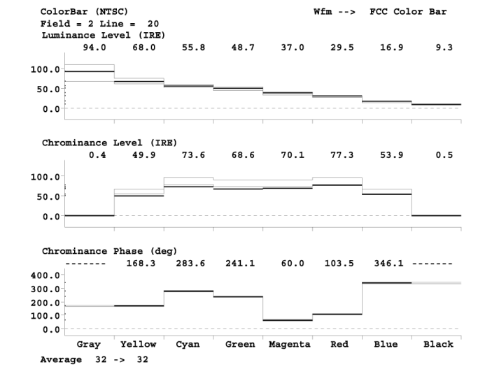
Color bar measurement.
