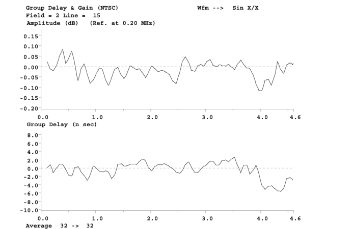
Frequency response and group delay measurement using Sin x/x.
