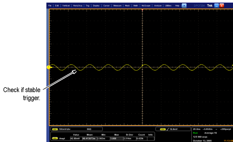
Figure 2-27: Measurement of trigger sensitivity - 50 MHz results shown
