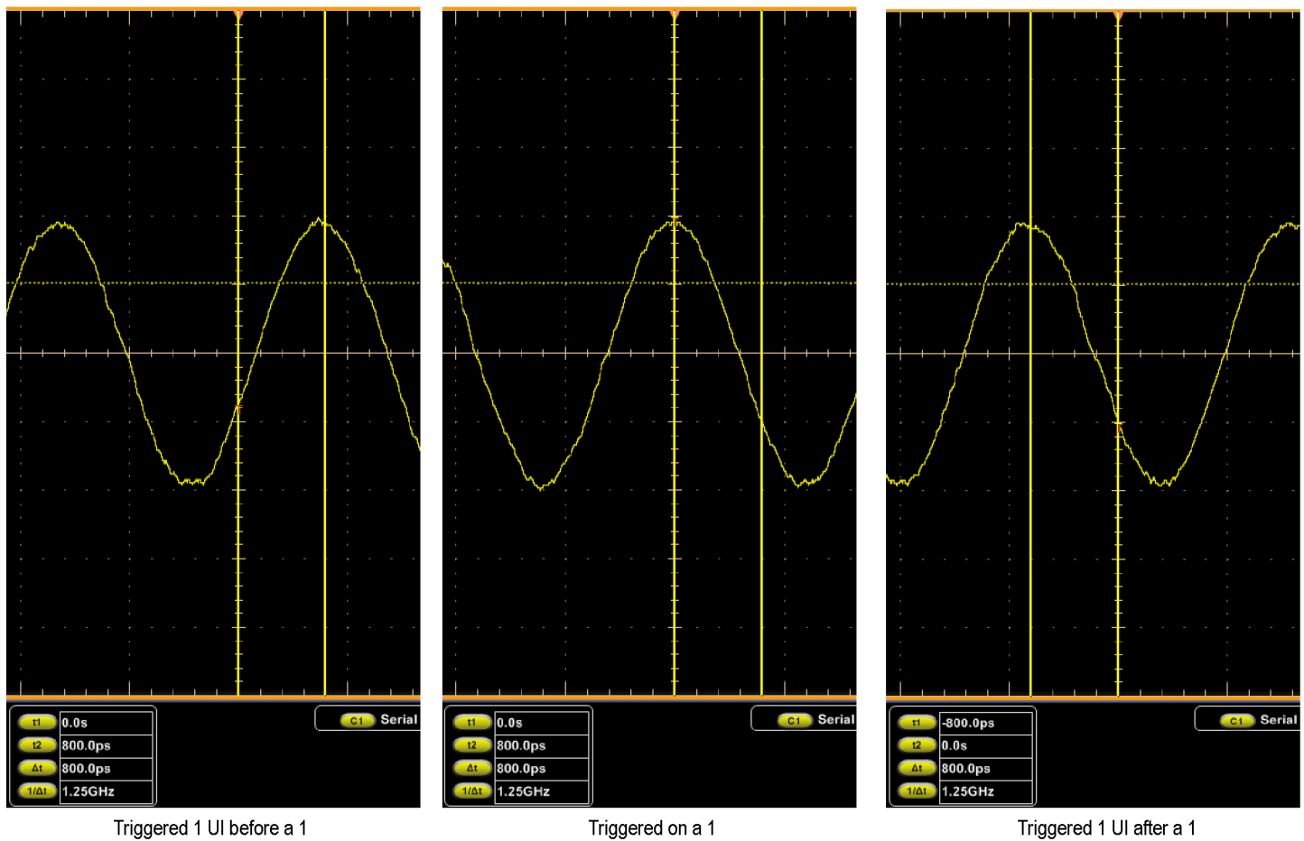
Figure 2-36: Isolated 1 triggering
