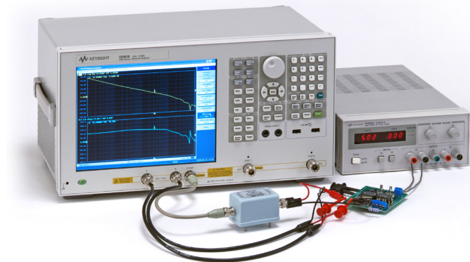
DC-DC converter loop-gain measurement with gain-phase test port
