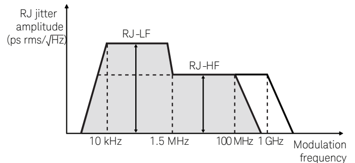
Figure 21. Spectrally distributed RJ allows to inject low frequency and high frequency RJ: this is required for compliant PCIe 2 receiver testing
