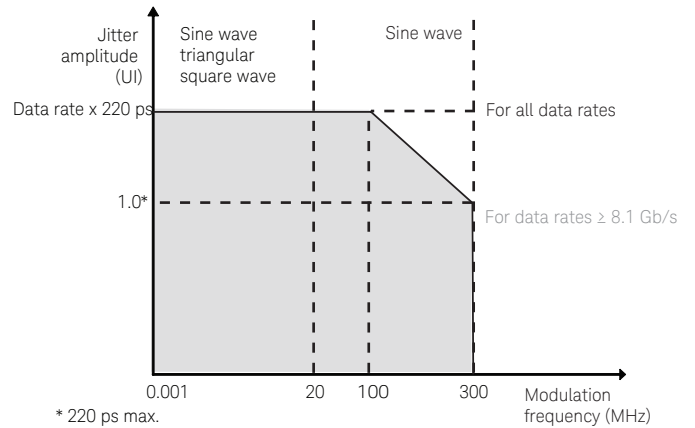
Figure 19. Periodic jitter maximum using the 220 ps delay line
